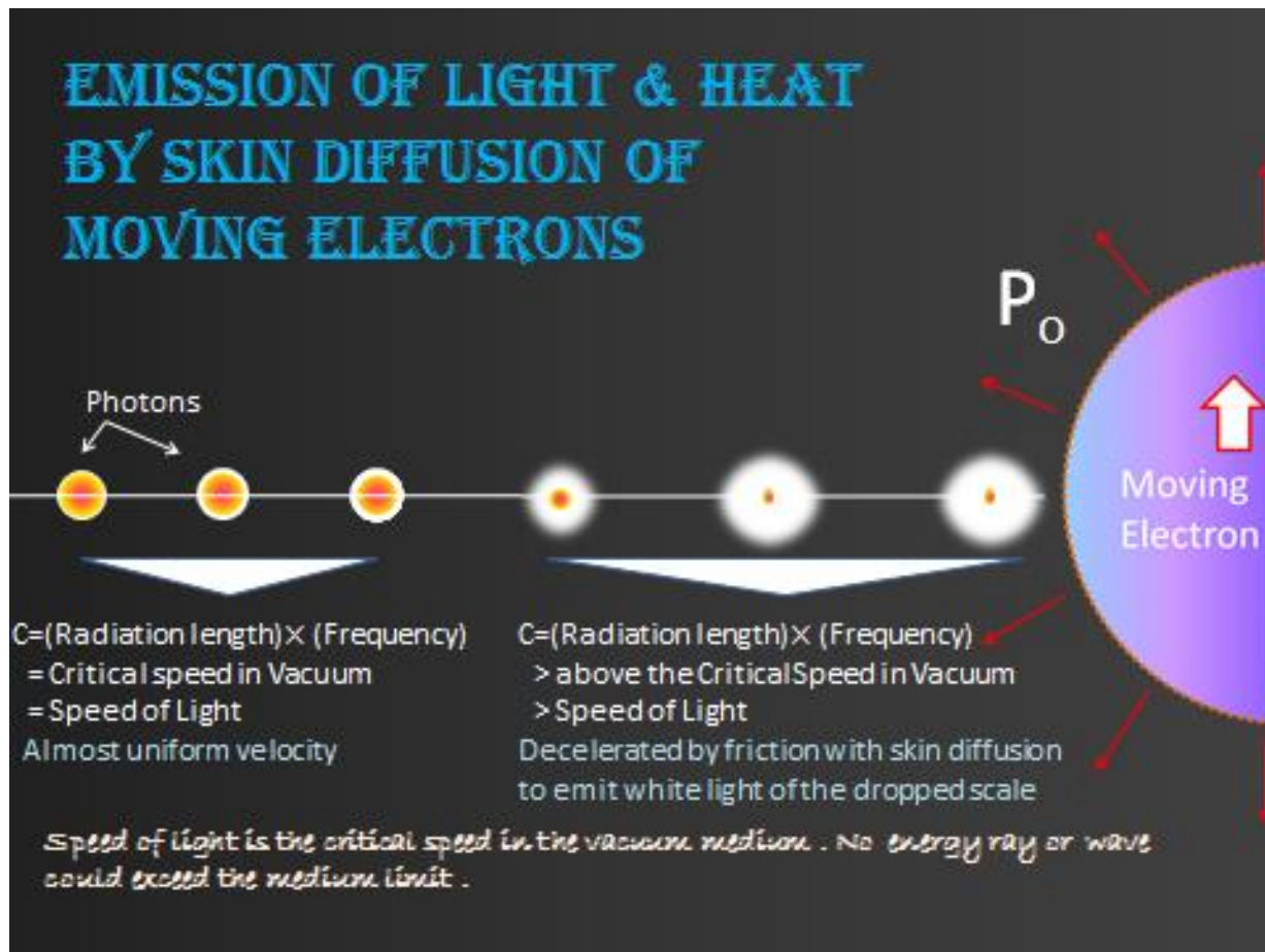
Figure-04 (Diffusion of Light and Heat from moving Electrons)
