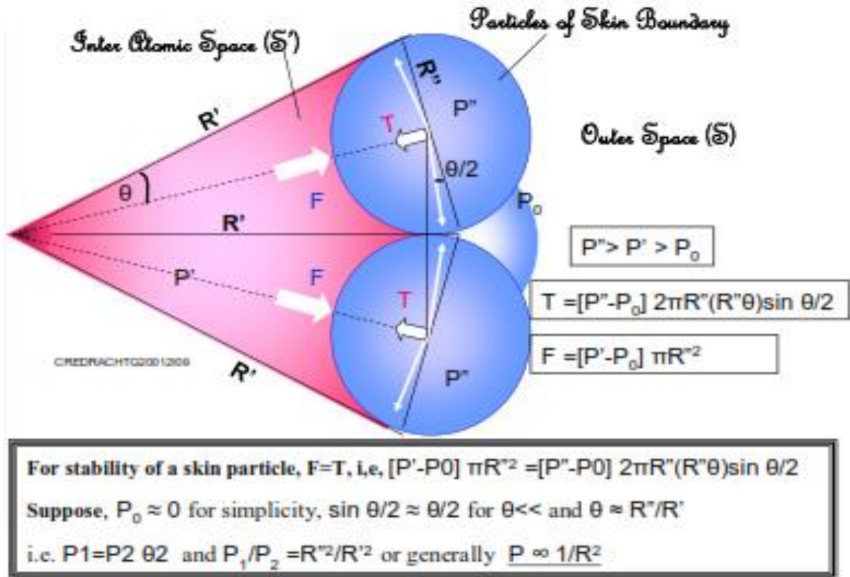
Figure-03 (Theory of skin tensioning of particles)
