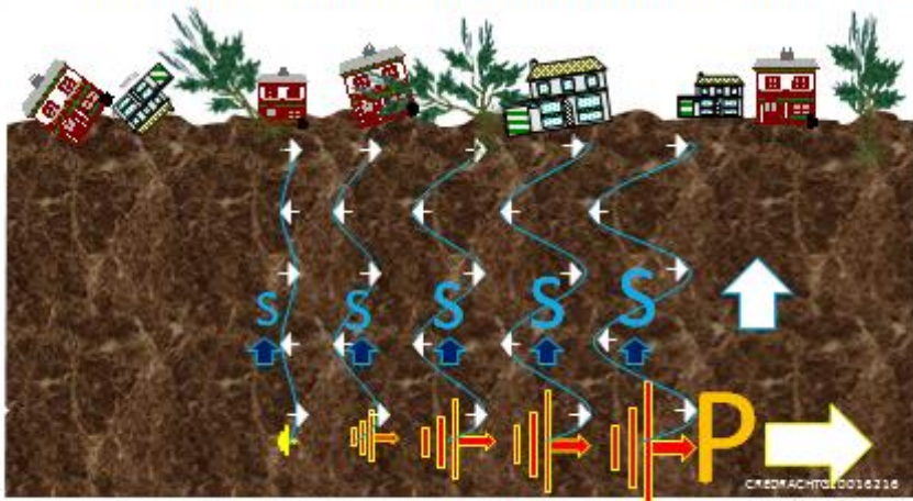
FIGURE-06 (Character difference between P-waves and S-waves)
