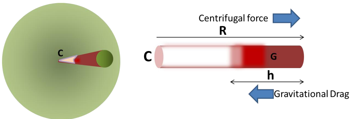
FIGURE-10 (Deduction on Material depth in Earth)
