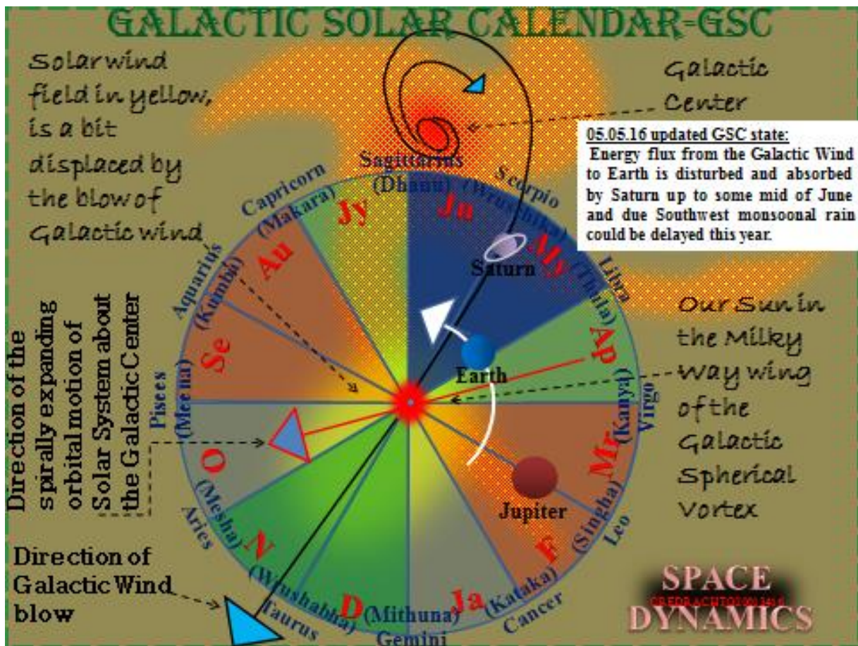
FIGURE-12(Galactic Solar Calendar to forecast changes in global climate &weather pattern)
