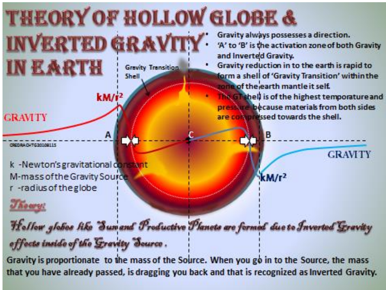
FIGURE-09(Gravity profile inside of Earth)
