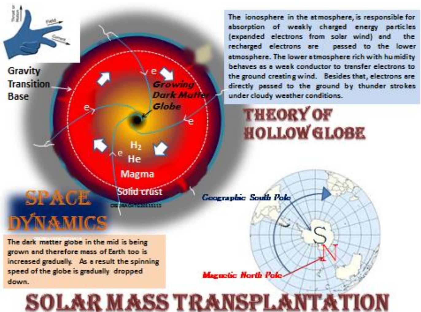
FIGURE-11(dark matter globe grown in the mid is common for all the Productive Planets)
